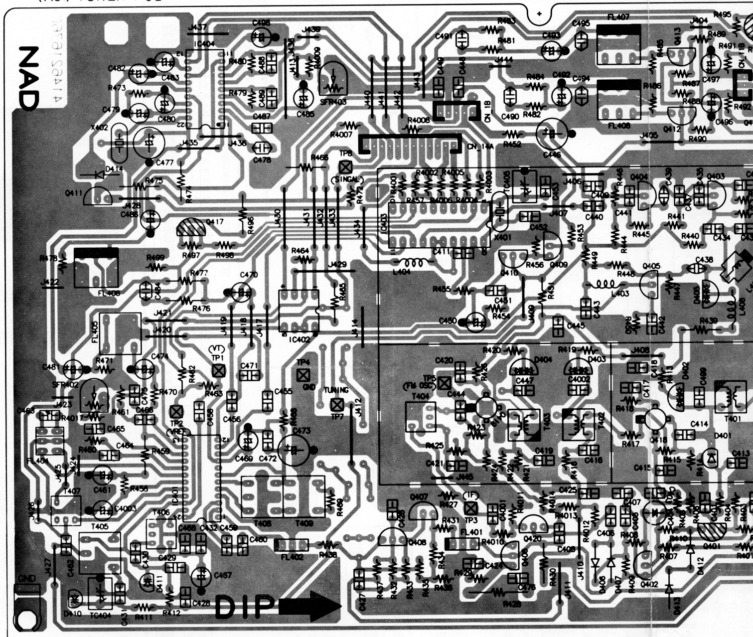
(M51) TUNER PCB
